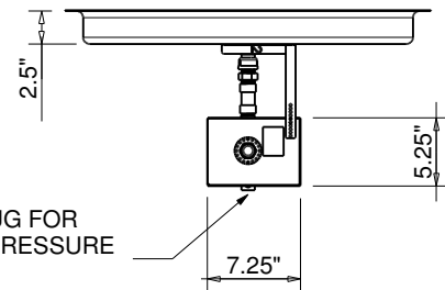
SIDE ELEVATION
